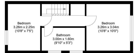
First Floor
